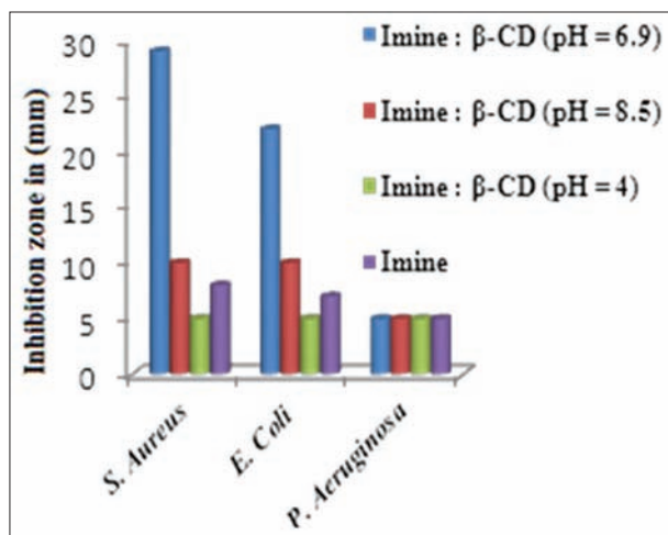
Figure 11: Histogram of free imine inhibition diameters and complexes at different pH
